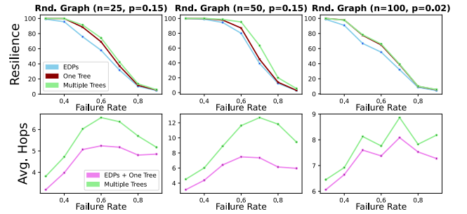
Figure 2: Random graphs with clustered failures.
