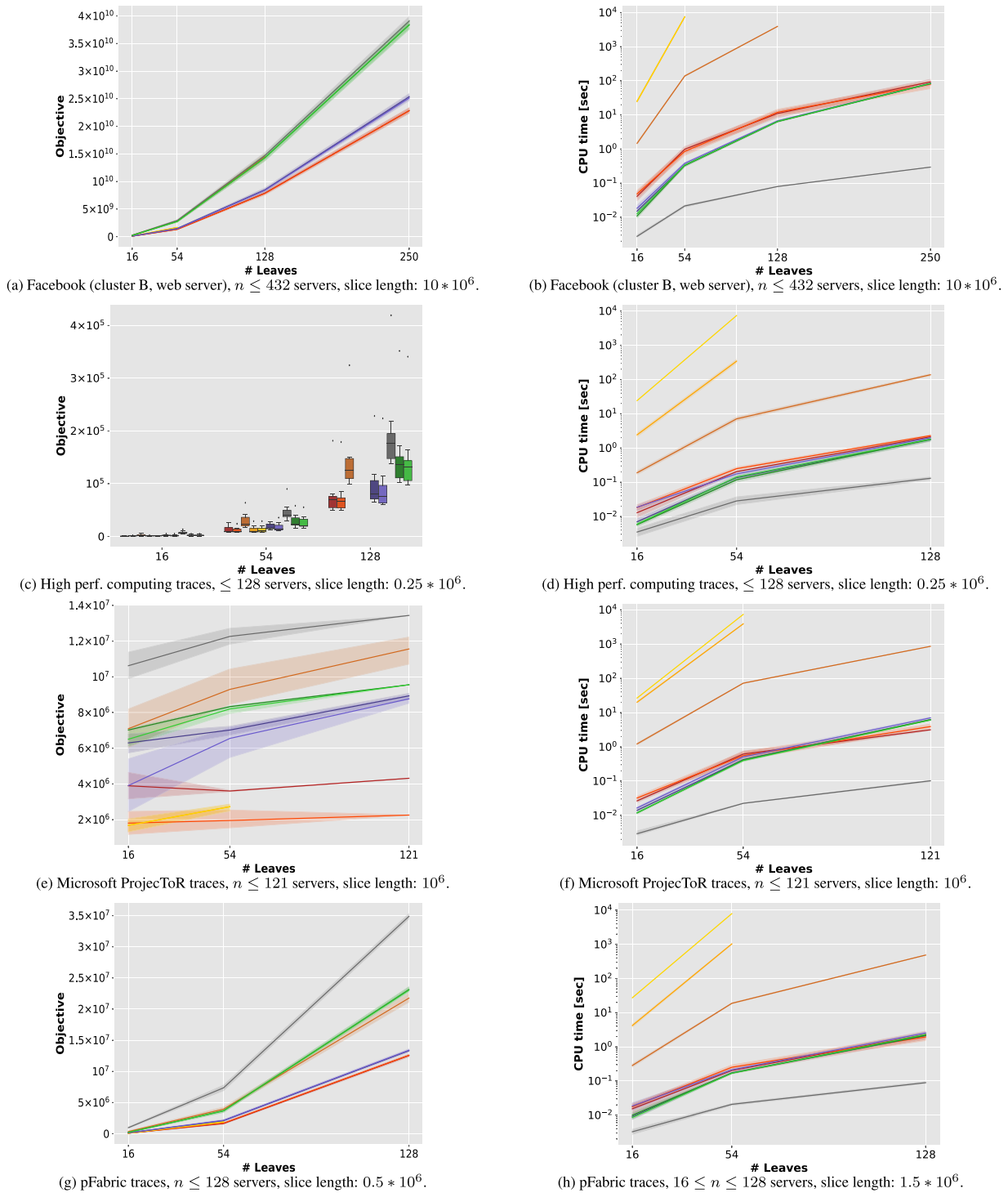
Fig. 4. Comparison of the different algorithms regarding objective value and CPU time.
