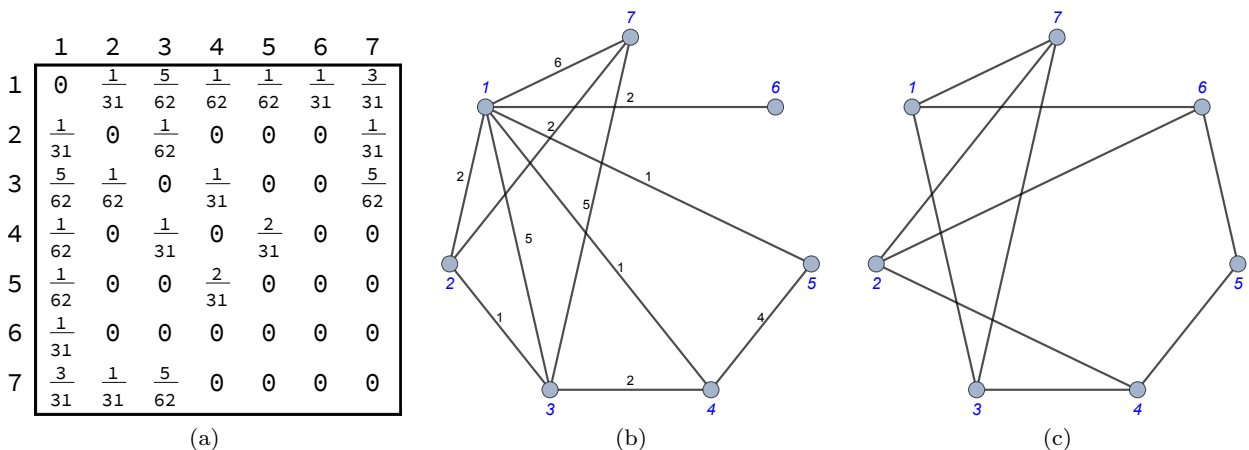
Fig. 1 Example of the bounded network design problem. (a) A given demand distribution \mathcal{D} (which in this case is symmetric ). (b) The demand graph G_{\mathcal{D}} (with non-normalized weights). Nodes 1 and 3 have a degree more than 3. (c) An optimal solution DAN N with \Delta = 3 . In this case, the solution is not a subgraph but contains auxiliary edges (e.g., \{5, 6\} ), and \text{EPL}(\mathcal{D}, N) = 1.16 while H(X | Y) = 1.02 (the Shannon entropy to the base 3 is H(X) = 1.61 ).
