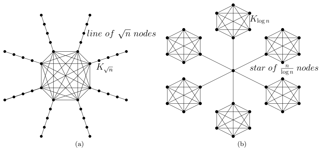
Fig. 3 (a) Different distortions on tree spanner w.r.t. different definitions. (b) Different distortion on tree network design (with auxiliary edges) w.r.t. different definitions
