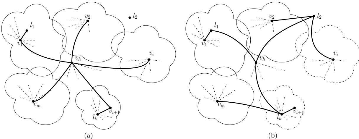
Fig. 2 (a) High out-degree node v_h in G has several edges to high in-degree neighbors. (b) v_h has only low degree neighbors, after using low degree helping nodes
