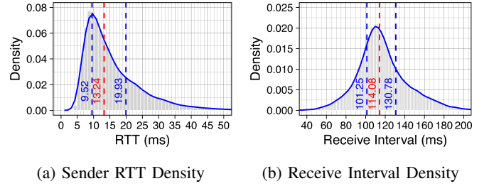
Fig. 6: RTT and Receive Interval Densities
