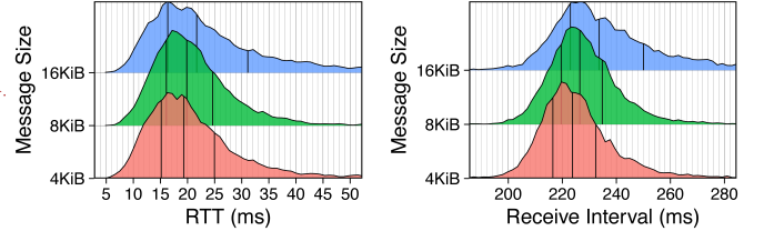
(a) Sender RTT Density over (b) Receive Interval Density over Message Size
