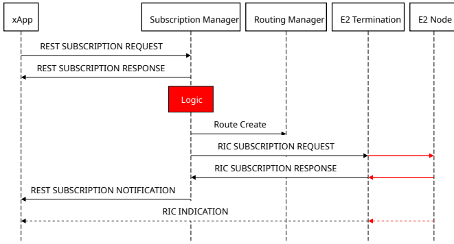
Fig. 2: Communication flow of a successful subscription request [7]
