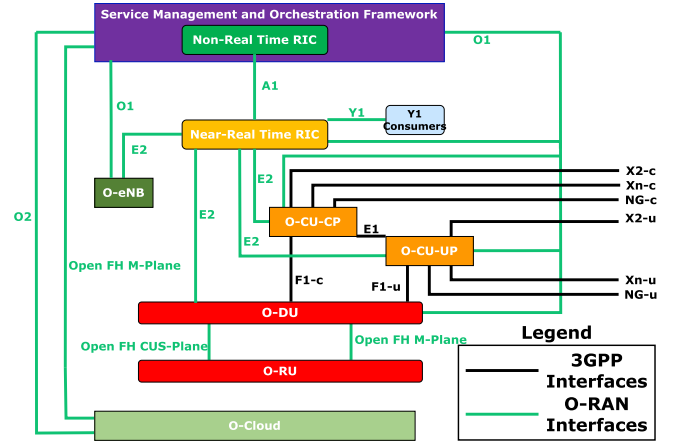
Fig. 1: O-RAN Architecture [1]
