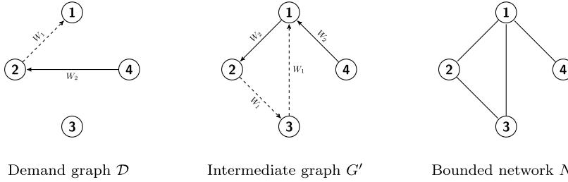
Fig. 1. In this example, \Delta_{avg} = 1 , thus the limit of the number of times a node can help is \lceil \Delta_{avg}/2 \rceil = 1 . Nodes 1 and 3 help the edges (4, 2) and (2, 1), respectively. For each node i , a Mehlhorn tree is built on the set of nodes that helped an edge connected to i . The initial degree of 3 is 0, thus there is no Mehlhorn tree from it. The Nodes 1 and 3 help the only edge of 4 and 1, respectively. Finally, 2 is connected to an outgoing and an incoming edge, thus two Mehlhorn trees including the nodes 1 and 3, will be built from 2.
