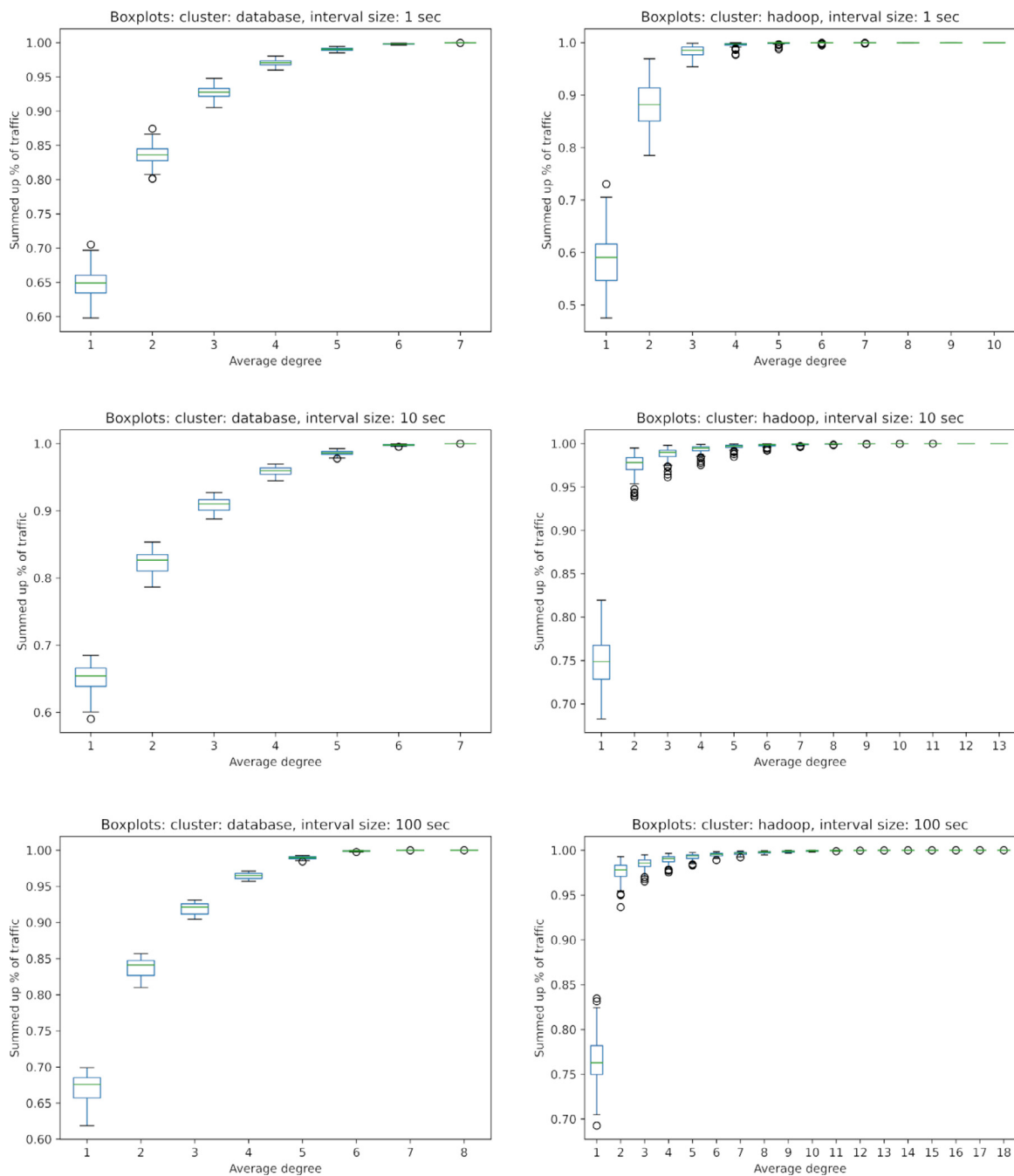
Fig. 2. Boxplots showing the % of traffic covered by different average degrees for Facebook’s database (left) and hadoop (right) cluster at the pod level, with 110 and 109 nodes, respectively.
