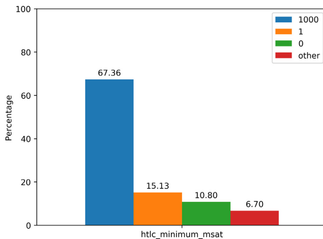
Fig. 3. htlc_minimum_msat distribution.
