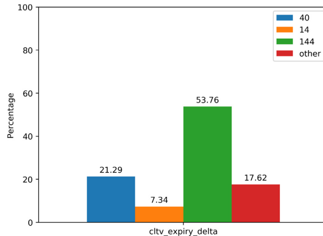
Fig. 1. cltv_expiry_delta distribution.
